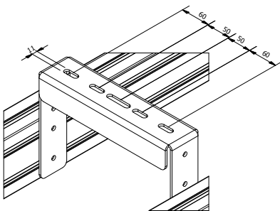
Fixing brackets
